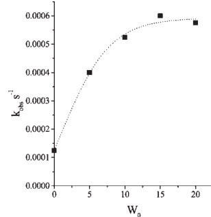
Figure 7. Variation of k_{\text{obs}} with W_0 in water–BHDC–benzene reverse micelles for the reaction of FNBA with PIP. [\text{FNBA}] = 1.5 \times 10^{-4} \text{ M} ; [\text{PIP}] = 0.1 \text{ M} ; [\text{BHDC}] = 0.2 \text{ M}
